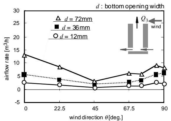
Figure 11 Airflow rate of top opening: Q_3
