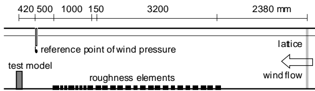
Figure 2 Wind tunnel geometry.
