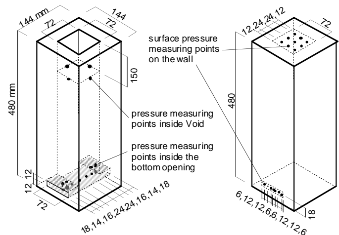
Figure 1 1/250 scale experimental model.
