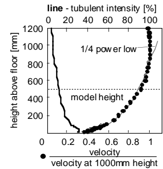
Figure 3 Approaching wind profiles.
