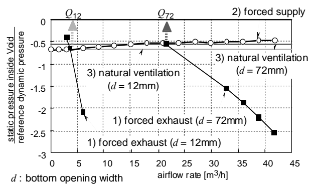
Figure 5 Variation of static pressure with airflow rate inside Void for one opening model.
