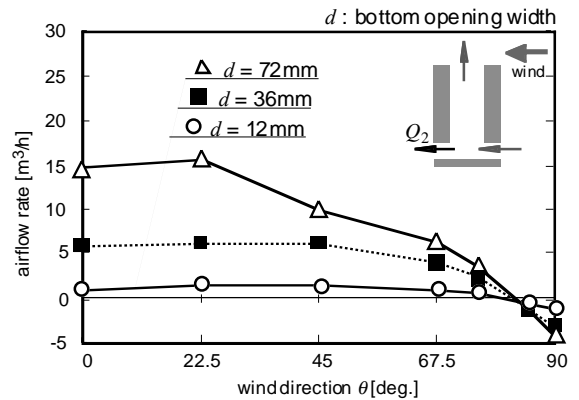
Figure 10 Airflow rate of leeward bottom opening: Q_2
