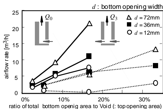
Figure 12 Airflow rate of Void: Q_0 vs Q_3
