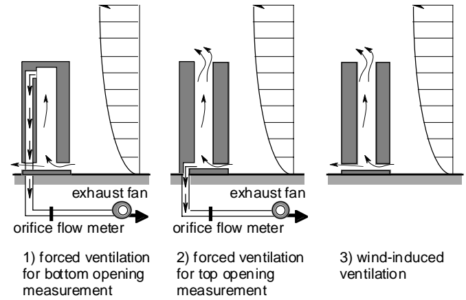
Figure 6 Airflow rate measurement of two openings model.
