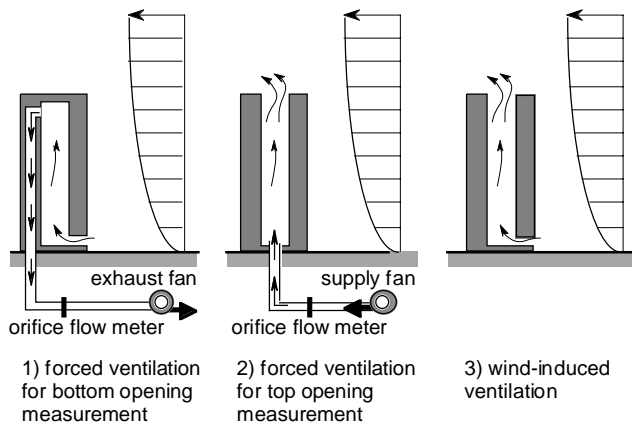
Figure 4 Airflow rate measurement of one opening model.
