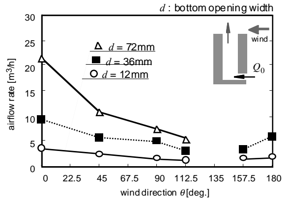
Figure 8 Airflow rate of bottom opening of one opening model: Q_0
