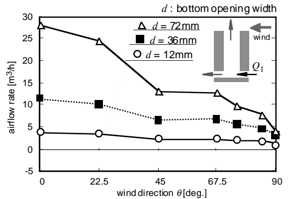
Figure 9 Airflow rate of windward bottom opening: Q_1
